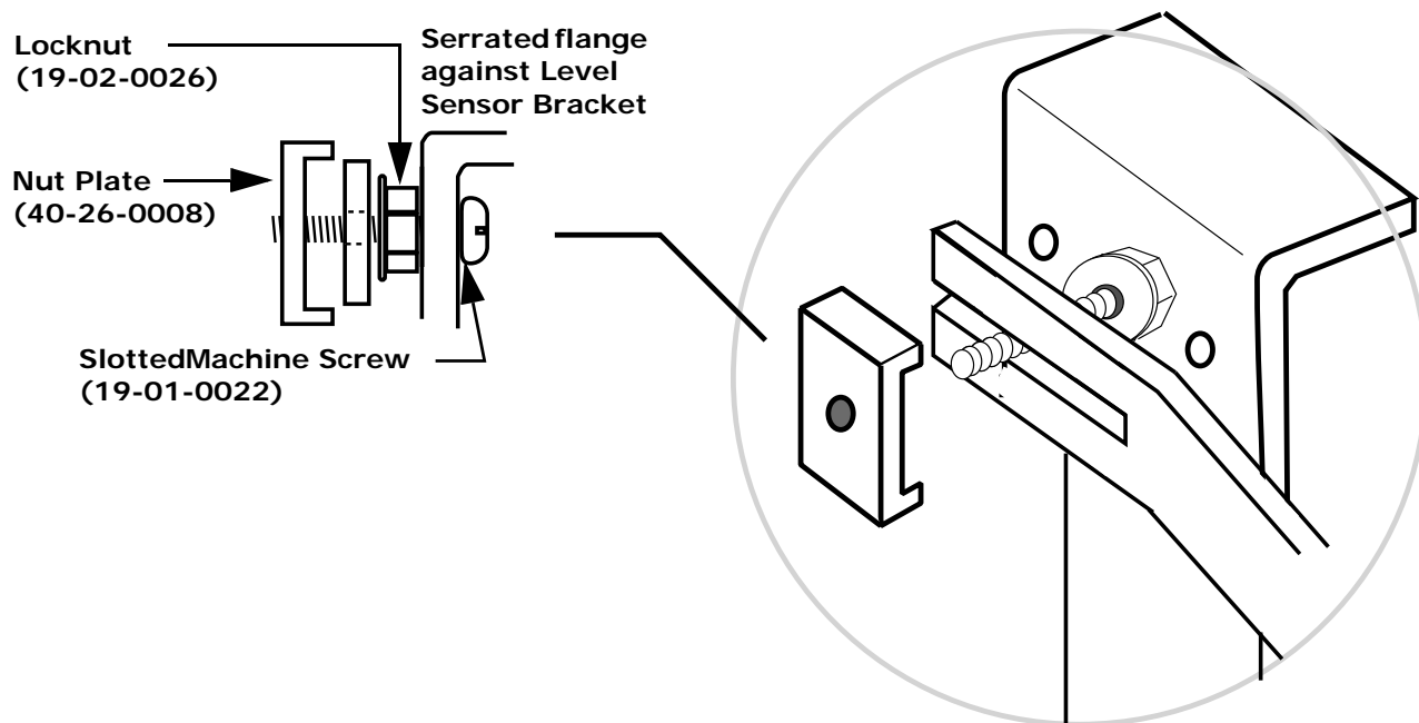
Figure 12. Level Sensor Mounting Hardware
