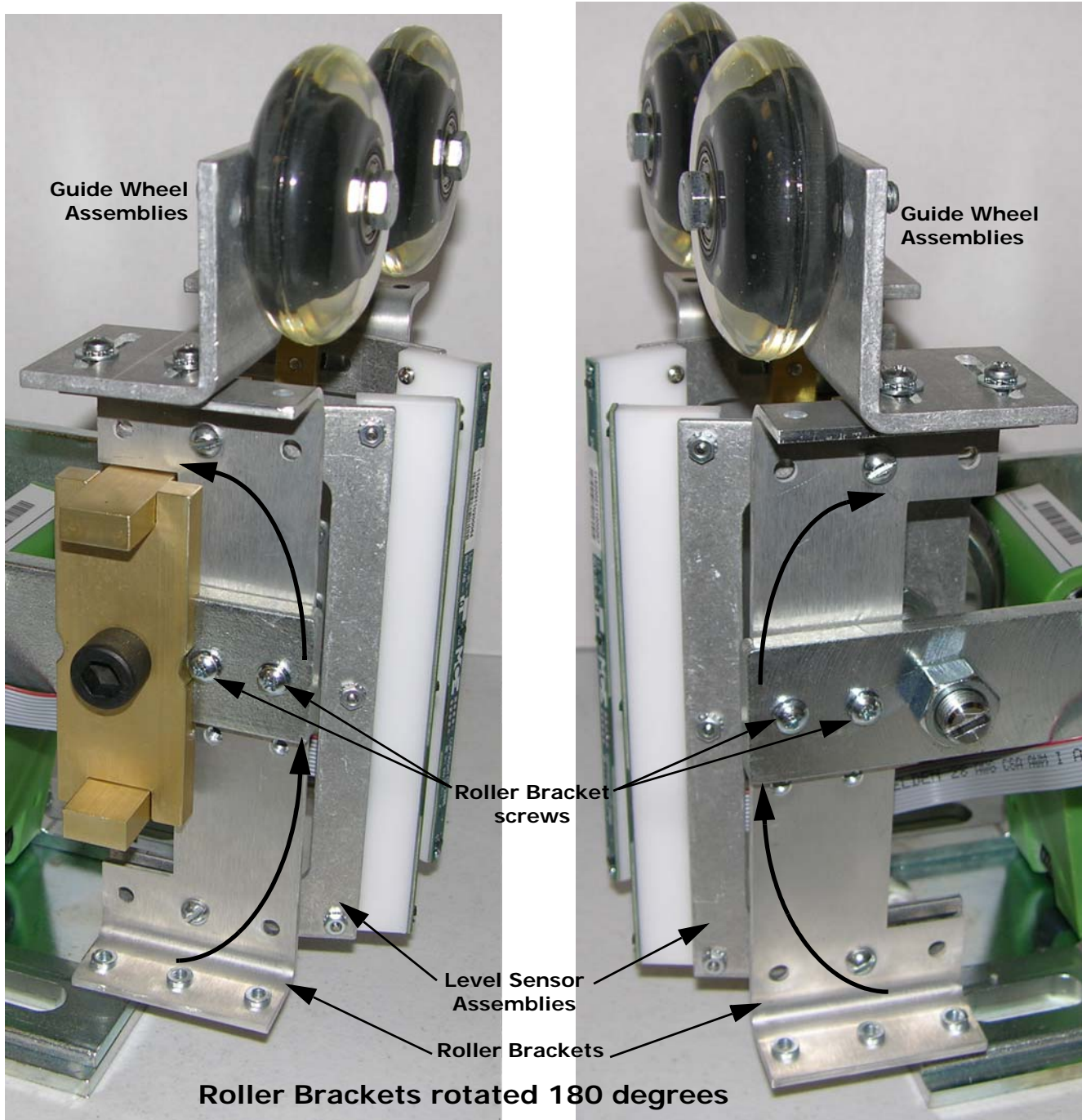
Figure 11. iLand Compact After Adjustment for Light Rail Use
