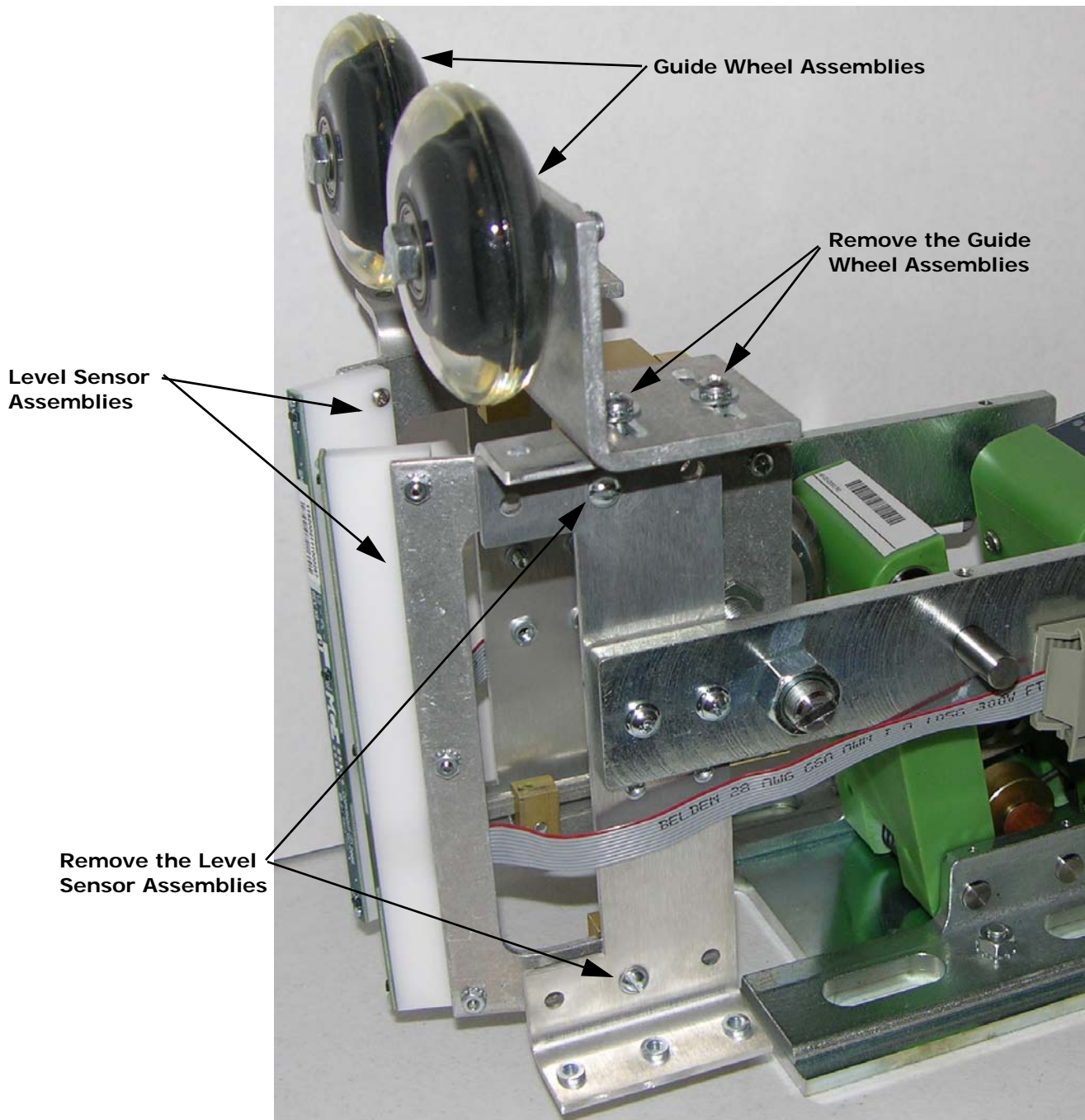
Figure 10. iLand Compact Standard Before Adjustment
