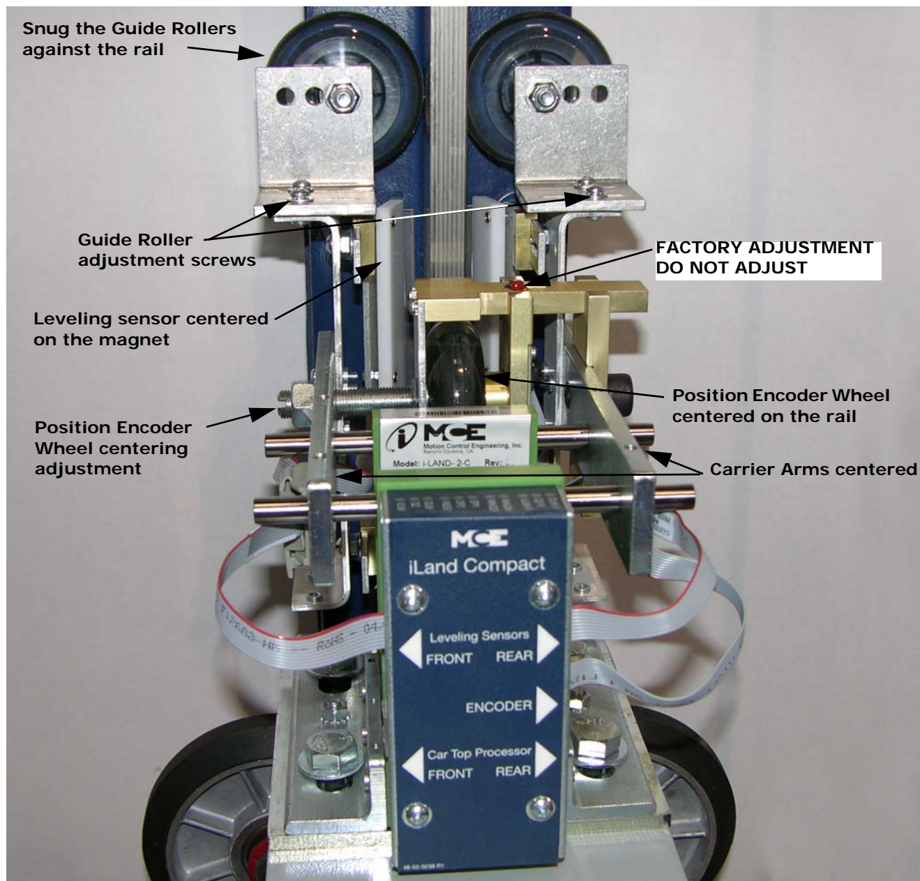
Figure 6. iLand Compact Installation (rear view)
