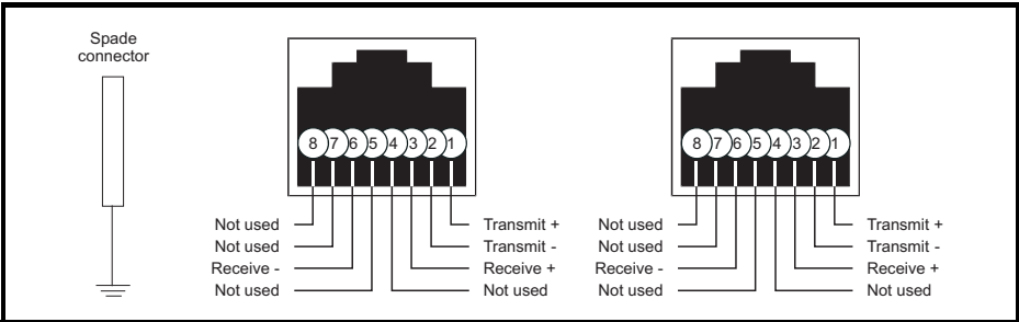
Figure 4-2 Ethernet connections
