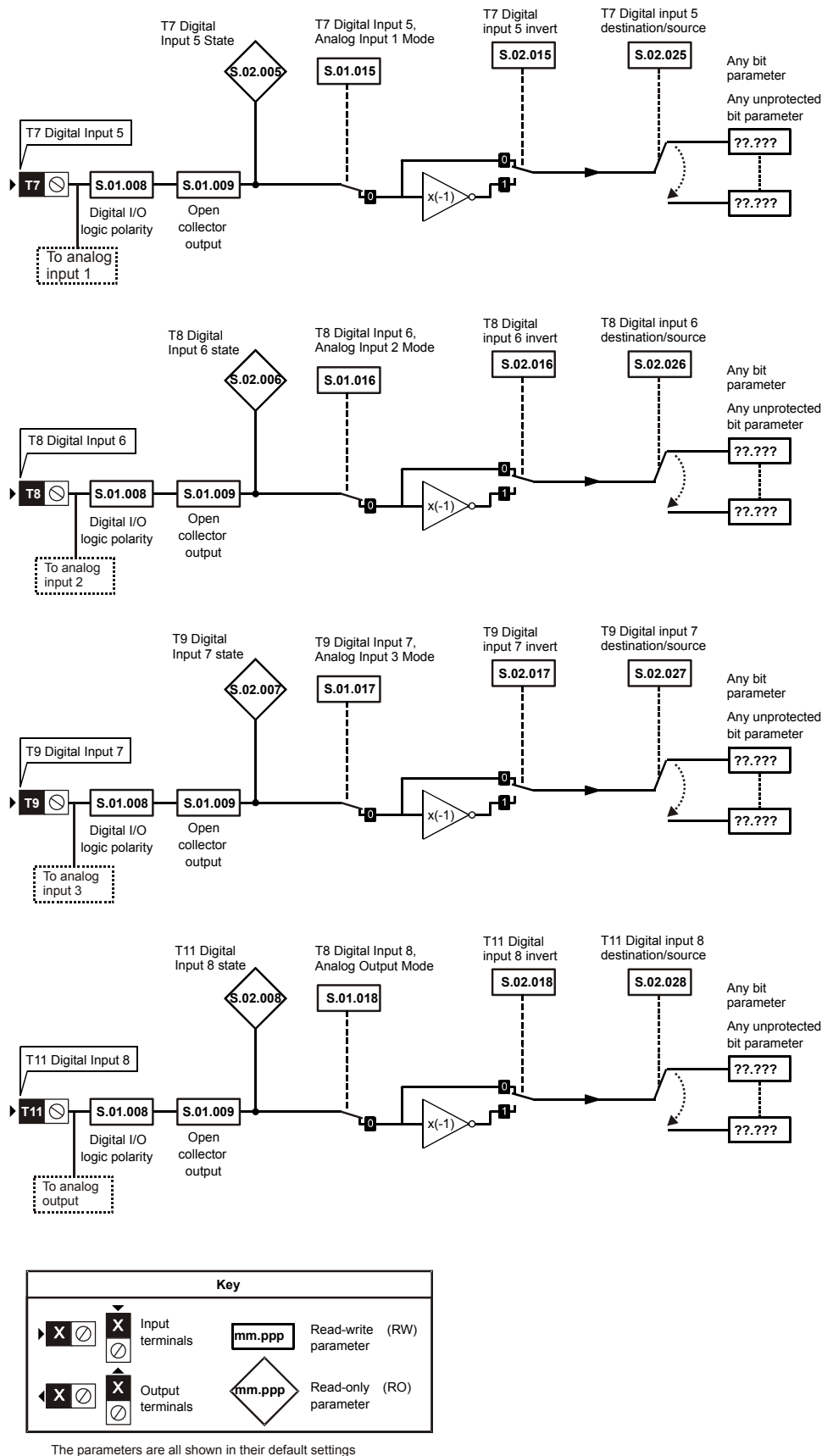
Figure 8-3 Digital input 5/6/7/8
