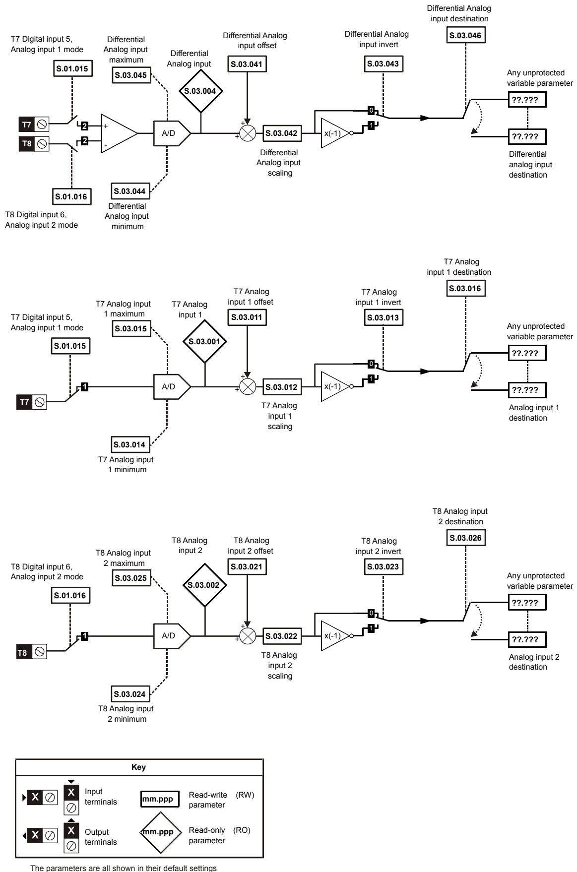
Figure 8-4 Analog input 1/2, differential analog input
