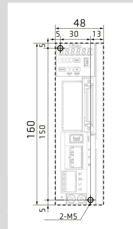
Mounting Dimensions
