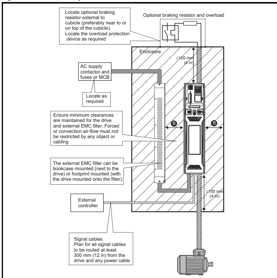
Figure 3-11 Enclosure layout
