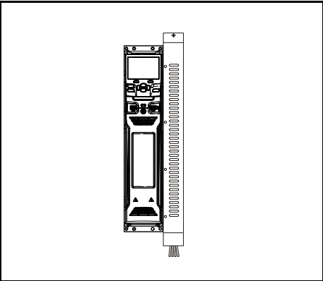
Figure 3-22 Bookcase mounting the EMC filter
