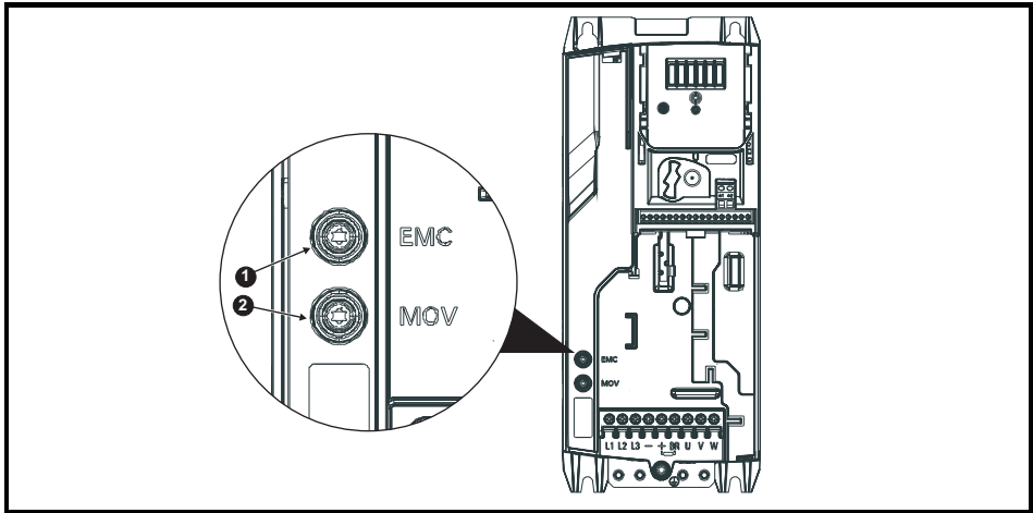
Figure 4-16 Removal of the size 4 internal EMC filter
