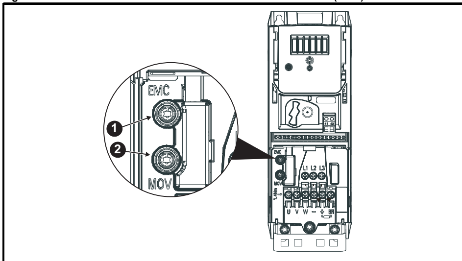
Figure 4-14 Removal of the size 2 internal EMC filter and Varistor (MOV)
