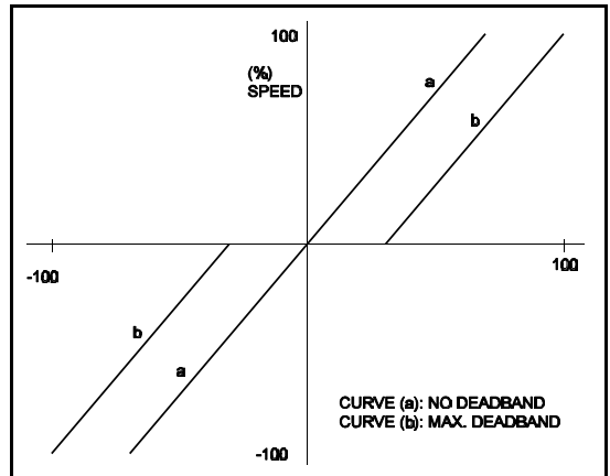
FIG. 10 – DEADBAND TRIMPOT ADJUSTMENT
