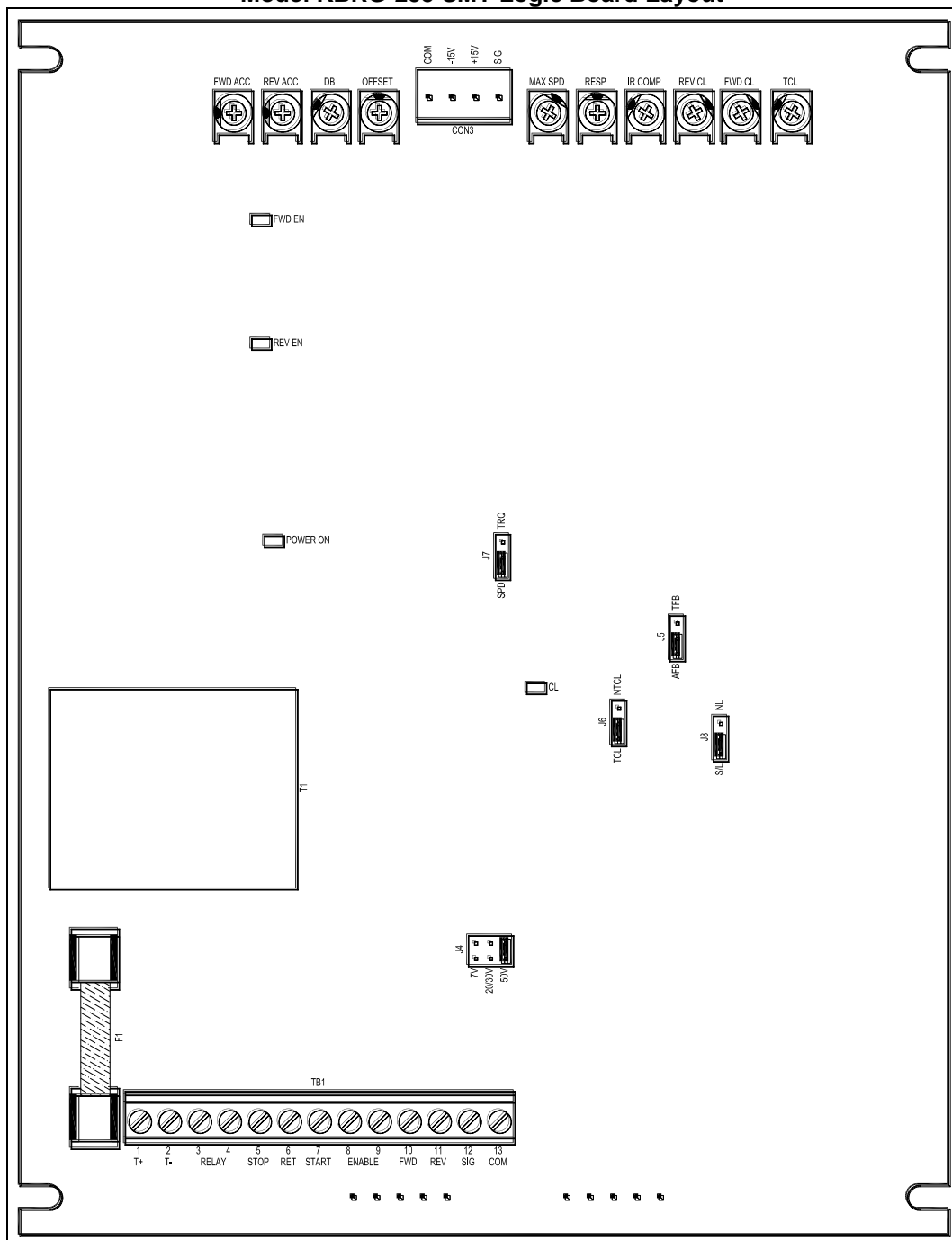
Model KBRG-255 SMT Logic Board Layout
