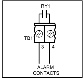
FIG. 7D – ALARM CONTACTS
