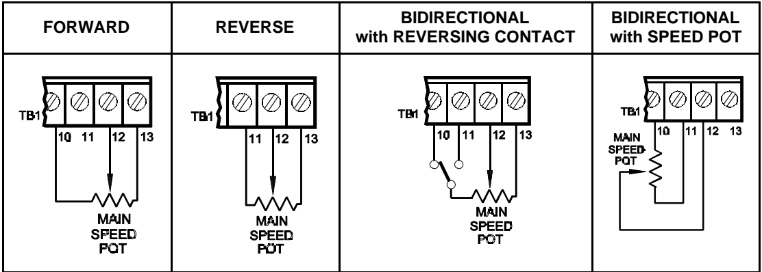
FIG. 7A – VOLTAGE FOLLOWING
