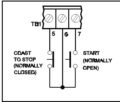
FIG. 7C – START/STOP CIRCUIT
