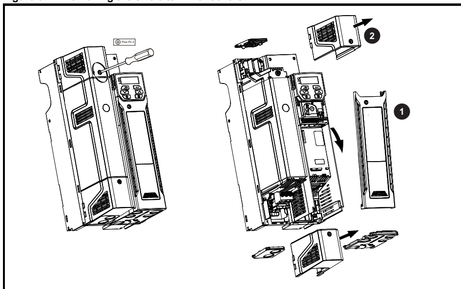
Figure 3-4 Removing the size 5 terminal covers
