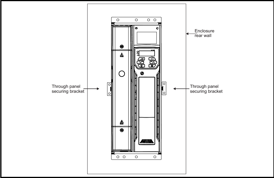
Figure 3-15 Through panel mounting
