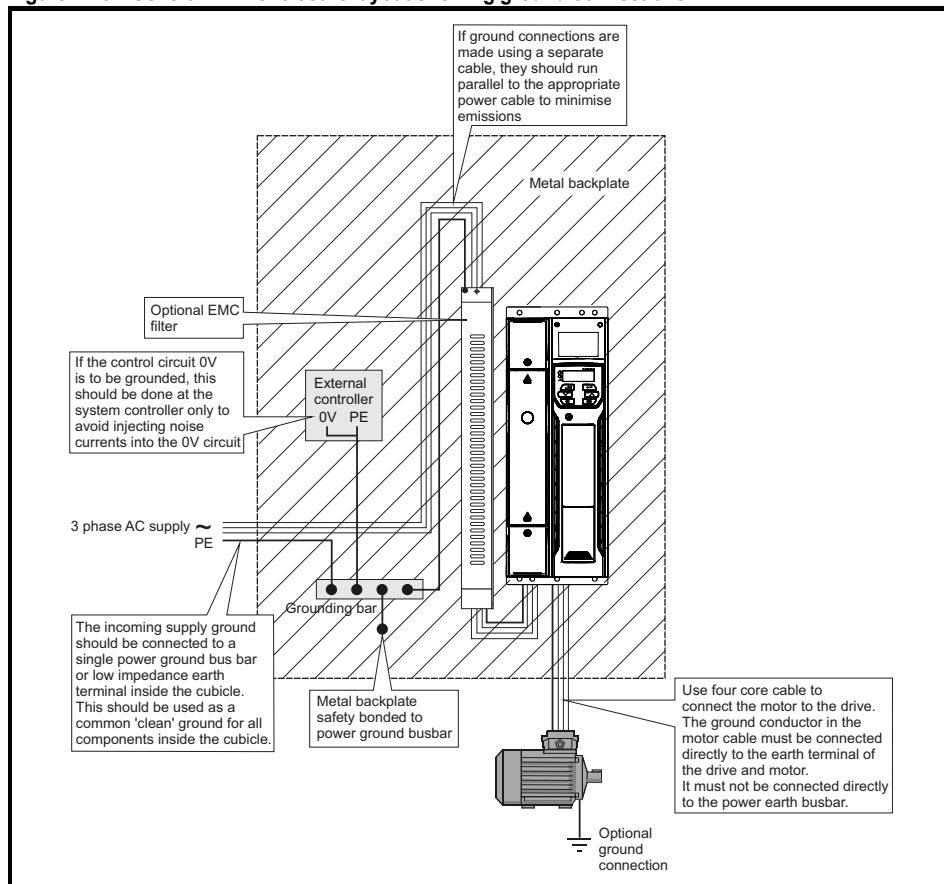
Figure 4-15 General EMC enclosure layout showing ground connections
