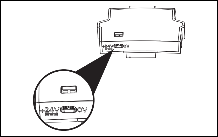
Figure 4-4 Location of the 24 Vdc power supply connection on the AI-Backup adaptor
