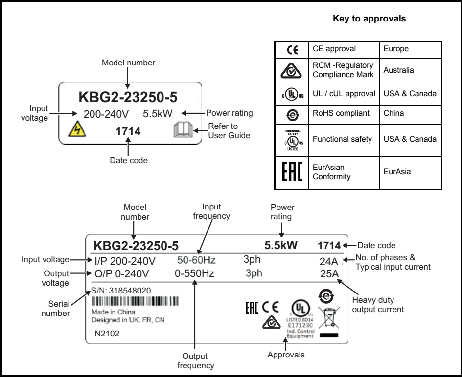
Figure 2-2 Typical drive rating labels (Unidrive M600 labels illustrated)
