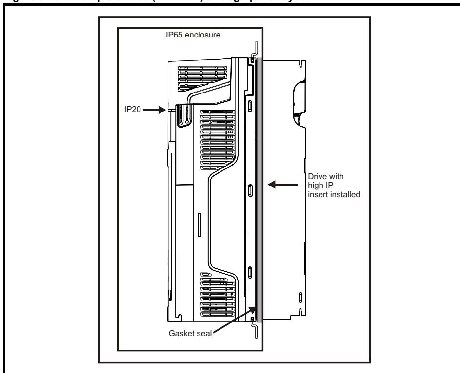
Figure 3-13 Example of IP65 (NEMA 12) through-panel layout
