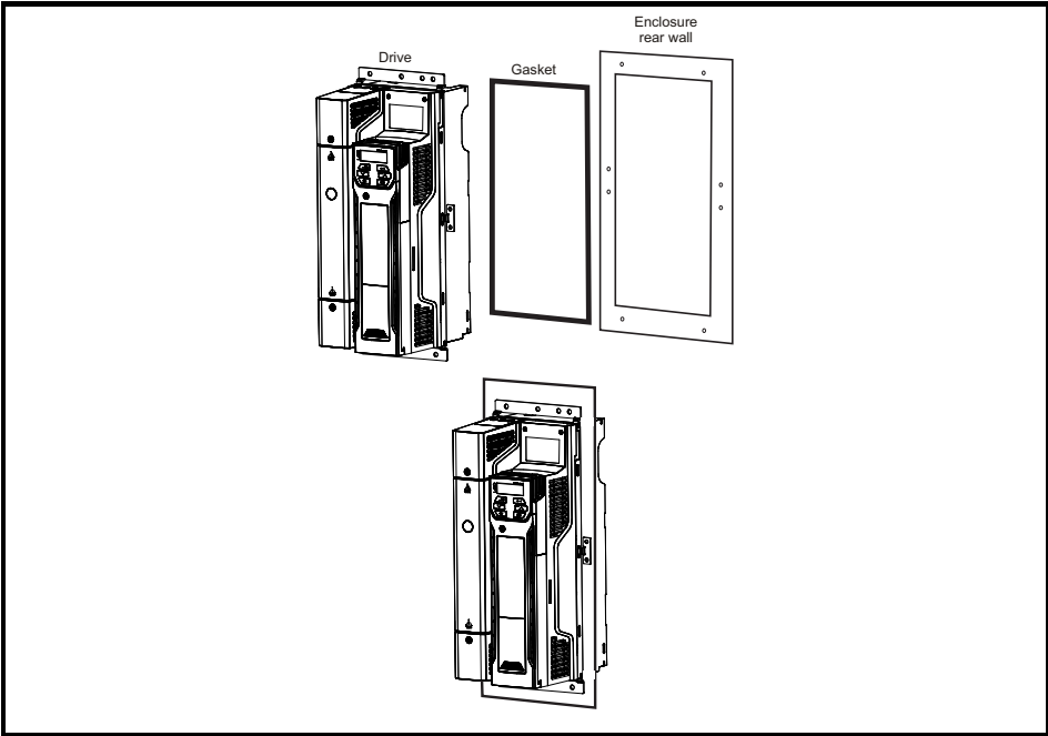
Figure 3-14 Installing the gasket
