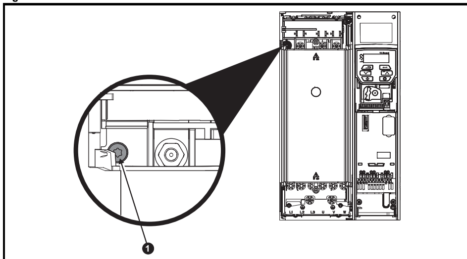
Figure 4-14 Removal of the size 6 internal EMC filter
