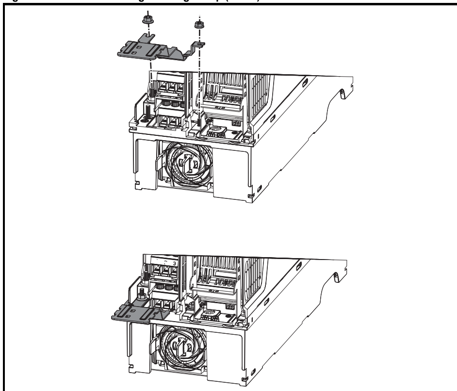
Figure 4-10 Installation of grounding clamp (size 5)
