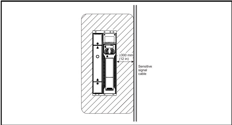
Figure 4-18 Sensitive signal circuit clearance
