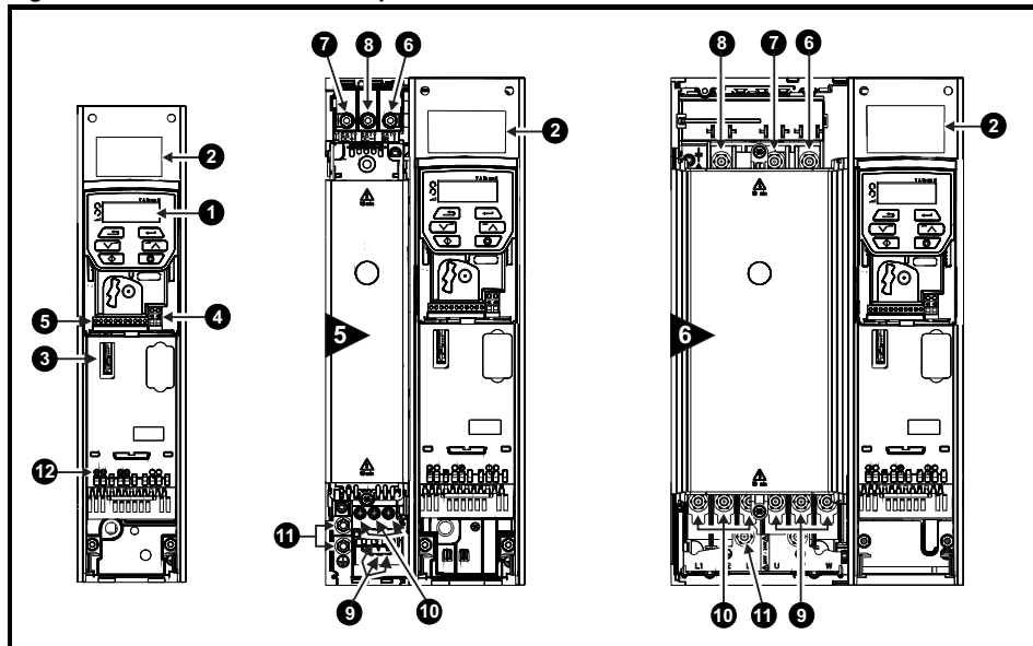
Figure 2-3 Features of the drive power section
