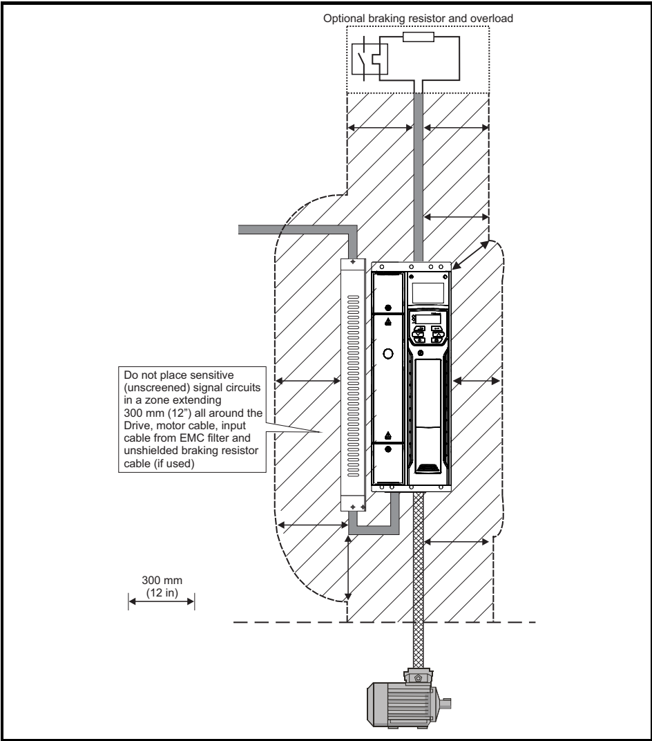
Figure 4-16 Drive cable clearances
