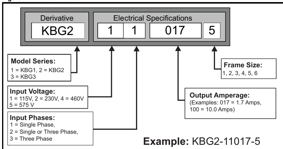
Figure 2-1 Model number
