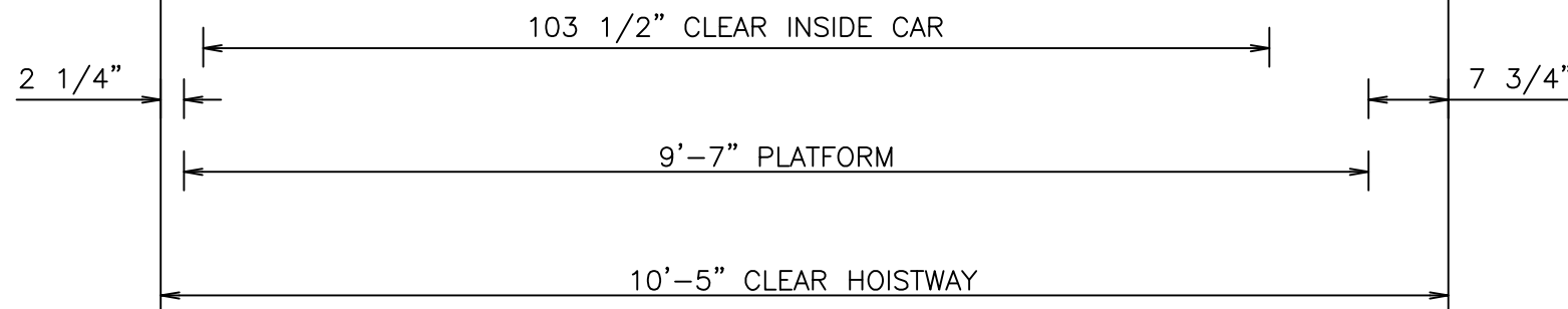
Plan View @ 1st SCALE : NONE (DEPICTING FEATURES AT VARIOUS LEVELS)
