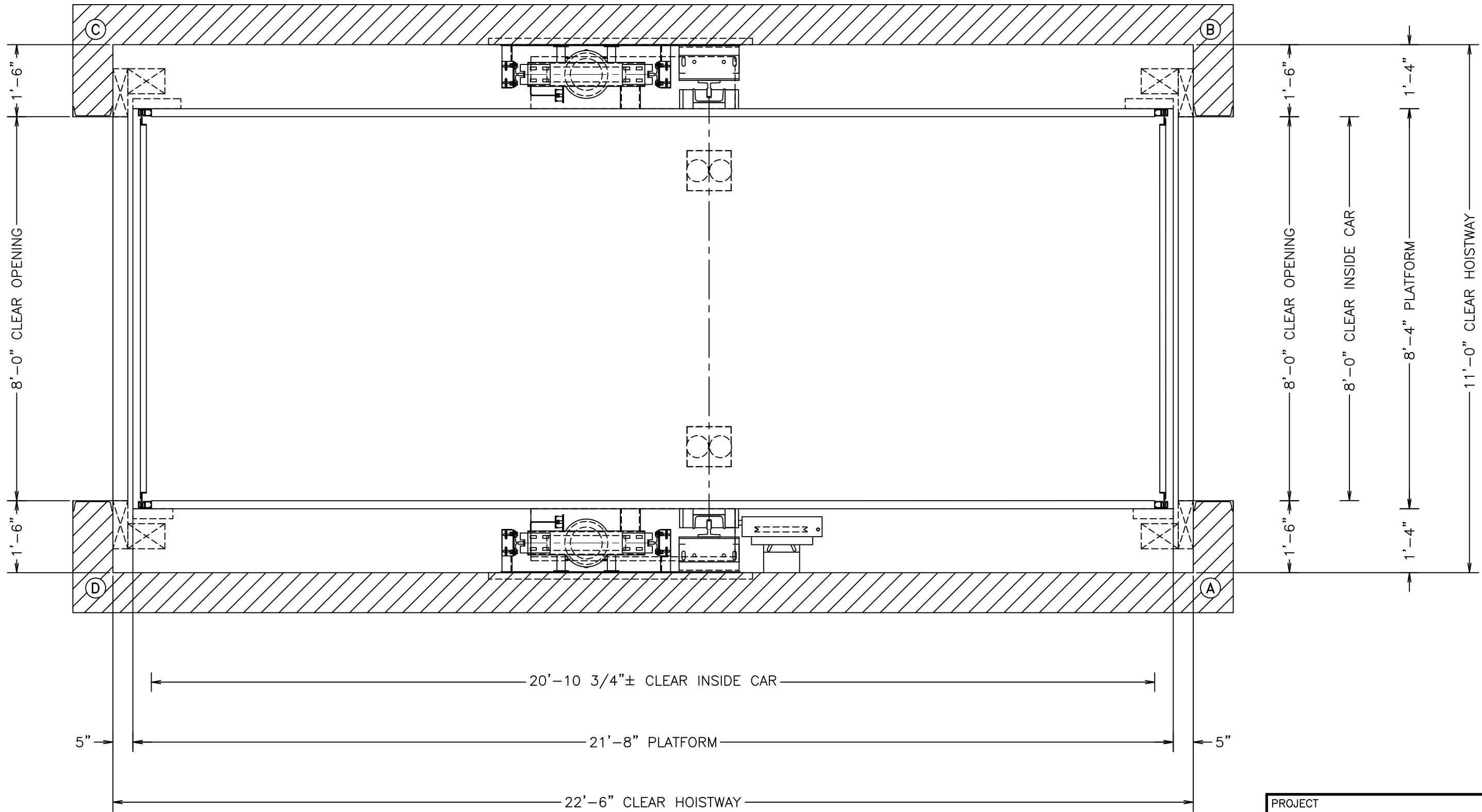
Plan View @ 1st Floor SCALE : NONE (DEPICTING FEATURES AT VARIOUS LEVELS)
