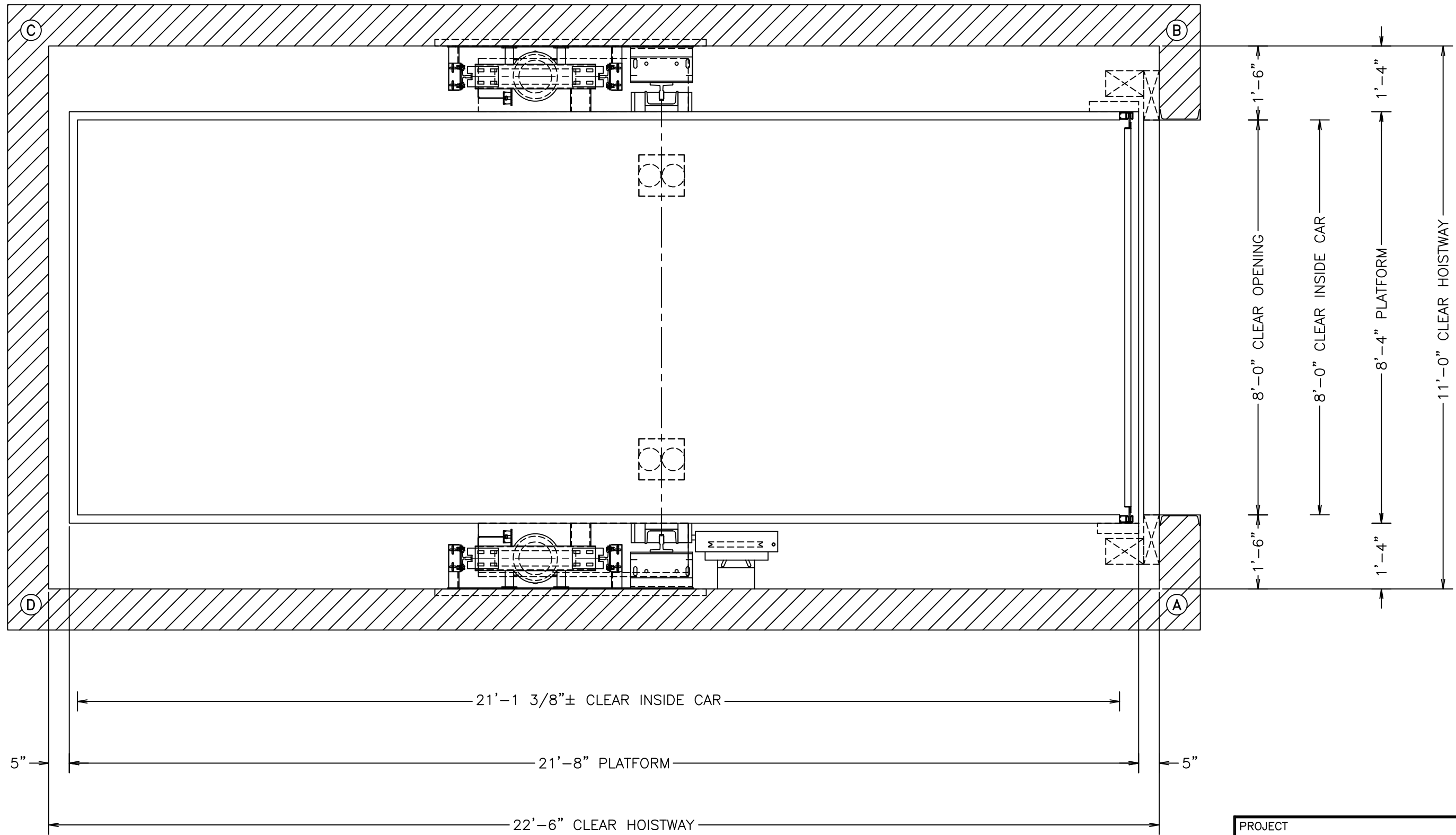
Plan View @ 1st Floor SCALE : NONE (DEPICTING FEATURES AT VARIOUS LEVELS)
