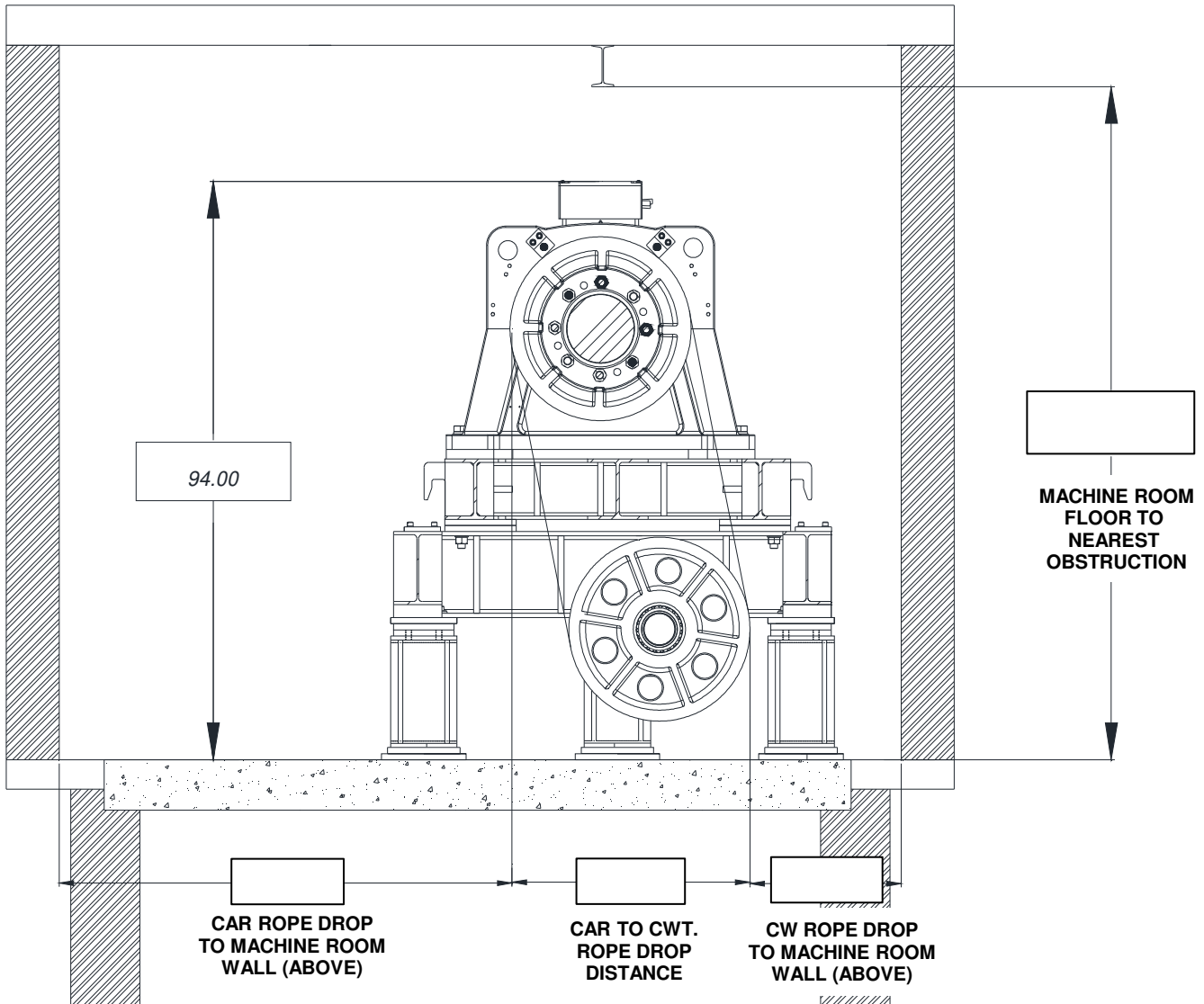
SKETCH D VIEW FACING THE MACHINE SHEAVE RIGHT-HAND SWING SHOWN
