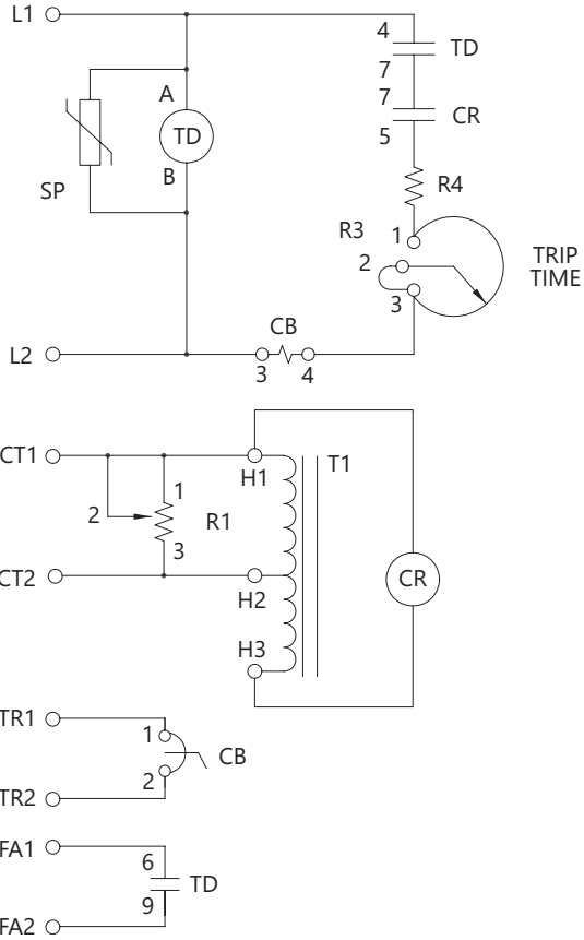
Figure 3: Electrical Schematic
