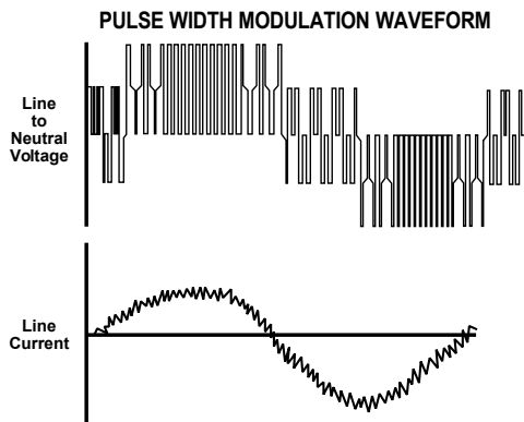
Figure 1 PWM Waveform
